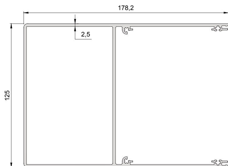
580-3101 ( 3,070 kg/mt ) SRA150 A05 STREAM PROFILE
