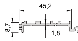
580-6205 ( 0,395 kg/mt ) REAR FINISH PROFILE
