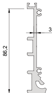
580-1204 ( 1,450 kg/mt ) SRA150M06 WALL FINISHING PROFILE
