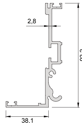
580-5102 ( 1,373 kg/mt ) SRA150 A10 TRANSMISSION PROFILE
