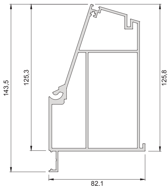
580-2101 ( 3,438 kg/mt ) SRA150 T01 CHASSIS PROFILE
