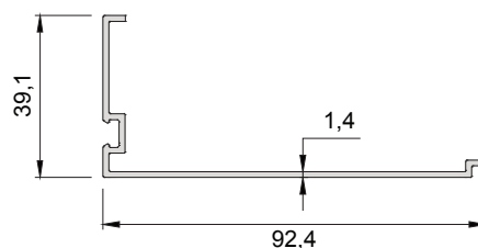
580-5103 ( 0,562 kg/mt ) SRA150 A11 FRONT CLOSING PROFILE
