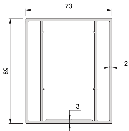
580-1201 ( 2,743 kg/mt ) SRA150 M03 CARRIER SEWING PROFILE
