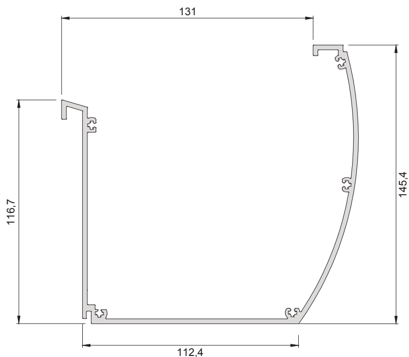
580-3101 ( 3,070 kg/mt ) SRA150 A05 STREAM PROFILE
