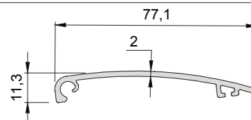
580-6205 ( 0,395 kg/mt ) REAR FINISH PROFILE
