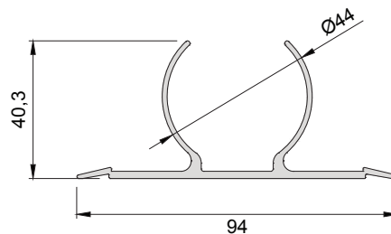
580-5101 ( 0,879 kg/mt ) SRA150 A09 CONNECTION PROFILE
