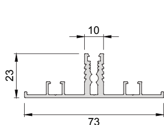
580-2101 ( 3,438 kg/mt ) SRA150 T01 CHASSIS PROFILE
