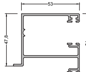
648-7101 (0,051 kg/mt ) ADAPTER PROFILE
