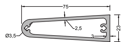
420-6010 (1,330 kg/mt) ADAPTER PROFILE
