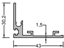
420-6001 (0,491 kg/mt) GSA130 ADAPTER PROFILE
