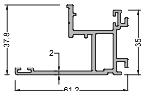
420-6005 (0,325 kg/mt ) ADAPTER PROFILE
