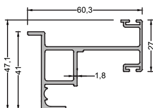
420-6007 (0,184 kg/mt ) ADAPTER PROFILE
