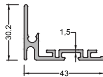
*420-6008 (0,504 kg/mt) GSA130 ADAPTER PROFILE
